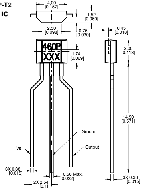
Figure 6. SS460P Sensor IC, SS460P-T2 Sensor IC and Ammopack Tape-in-Box Mounting Dimensions (For reference only. mm/in.)
