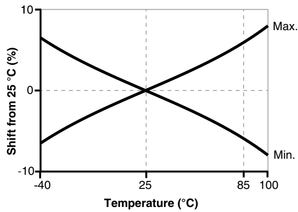
Null Shift vs Temperature
