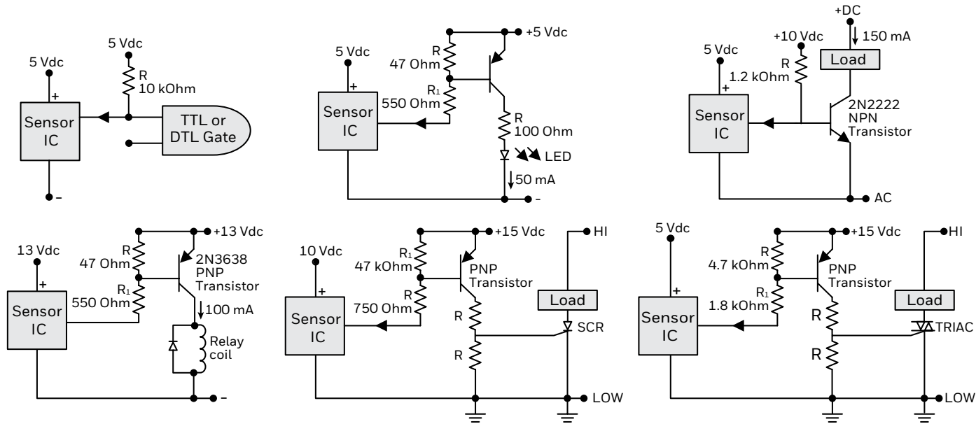
Figure 2. Wiring Diagrams
