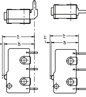
Operate Point References for PCB Terminals
