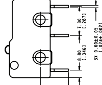
Terminal Type 20 - Straight PCB
